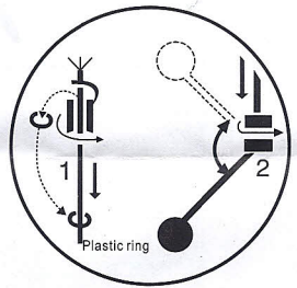
Fig.8:Peel the plastic ring off the counterweight before installation and setthering around the cable, then insert the cable from the conic part into the counterweight and fix it with moderate pressure at the fixing end.
